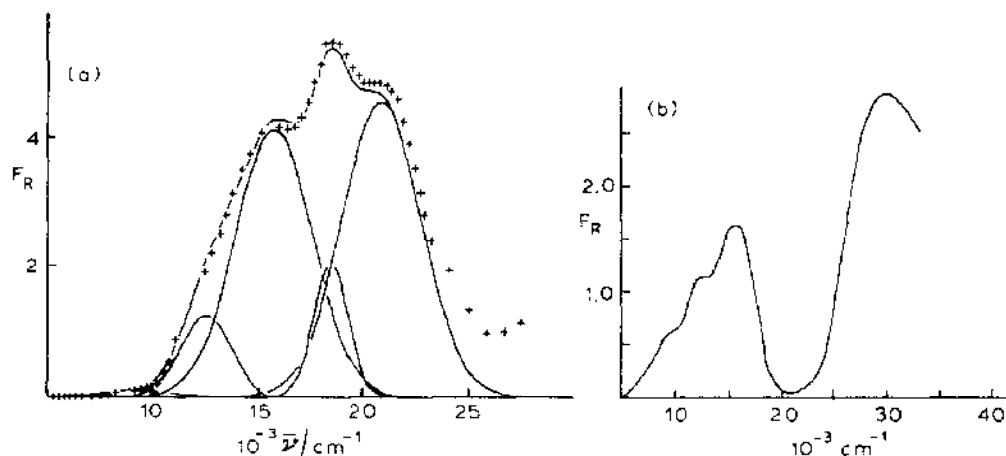
Fig. 17. Diffuse reflectance spectra of \text{Ba}[\text{AgF}_4] and \text{Ag}[\text{PbF}_6] from ref. 227.
